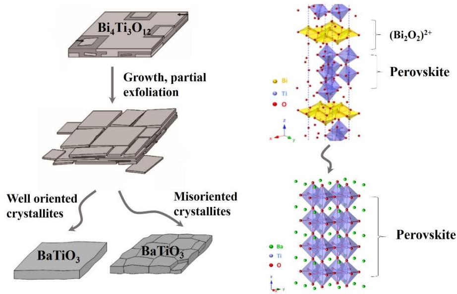
Figure 1.15 Schematic of preparing BaTiO 3 templates with the topochemical conversion reaction [69] .
