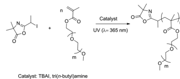
Scheme 2 Photo-polymerization of mPEGMA at \lambda = 365 \text{ nm} with I-Azl initiator and tri( n -butyl)amine or TBAI catalyst.
