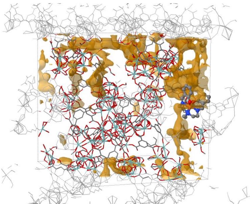
Figure 5. Reconstructed FES F(T; x_{\text{Ga}}, y_{\text{Ga}}, z_{\text{Ga}}) of 2 -MOF-808 obtained from the WT-MTD simulations performed at T = 350 K ( F = -50 mHa) superimposed with the optimized HS structure of 1 -MOF-808 obtained from the configuration 2 (see Text).
