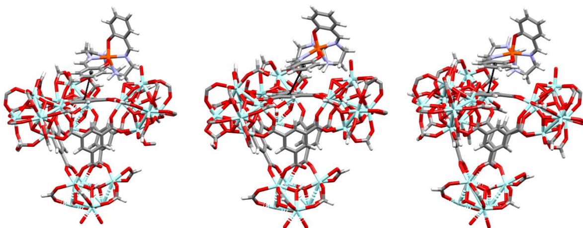
Figure 6. Snapshots of the structures of the three most stable minima of 1C -MOF-808 located on the estimate of the FES and further optimized by DFT, the shortest contacts between the MOF-808 linker and the SCO complex are evidenced by the black line.
