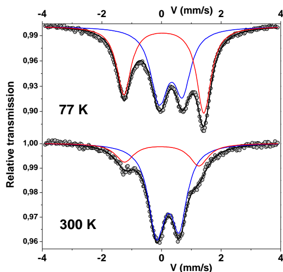
Figure 4. Mössbauer spectra of ^{57}\text{Fe} enriched 1@120nm-21% at 300 K and 77 K. The HS and LS components are in blue and red, respectively.
