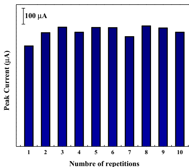
Fig. 9 Repeatability of Sn/SnO 2 in PBS (pH 6) containing 20.7 \mu\text{g L}^{-1} of Pb(II) under optimum conditions
