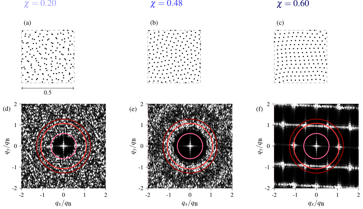
FIG. 2. (a,b,c) typical configurations of two-dimensional SHU point patterns for increasing values of the stealthiness ( \chi = 0.2, 0.48 , and 0.6 ), obtained as detailed in Ref. 28 . (d,e,f) corresponding structure factor S(\mathbf{q}) , as estimated by the spatial Fourier transform of a pattern having the dimensions (L, 1) of the slab in Fig. 1, with L = 3 (it is thus made of approximately 2000 scatterers). On each plot, the pink, red and dark red circumferences represent the chosen observation frequencies, k/k_B = 0.6, 1.08 , and 1.28 , see Fig. 3.
