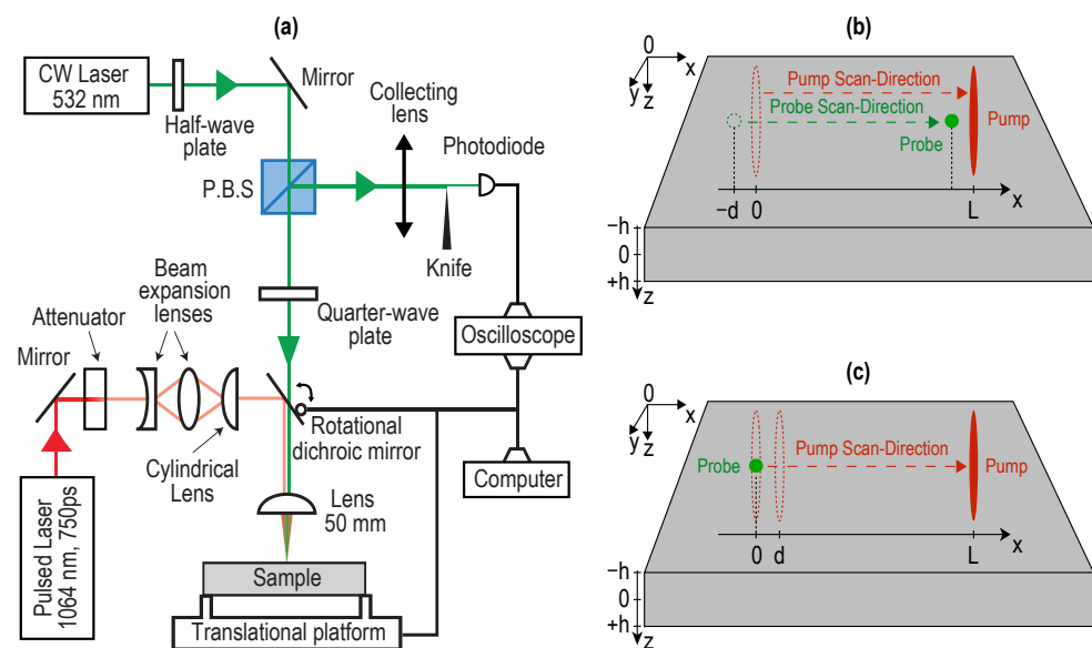
Figure 2. (a) Experimental setup. (b,c) Illustration of the two scanning configurations used: (b) the rotational mirror is fixed with d = 20 \mu\text{m} , and then the plate is moved along x -axis; (c) the plate is fixed, and the mirror rotates.
