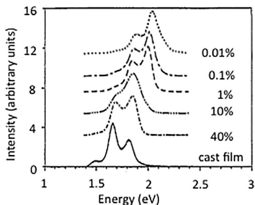
FIGURE 24 Photoluminescence spectra of PE/POT blends with different concentrations (wt%) of POT (excitation energy: 2.41 eV). Reproduced with permission. 39 Copyright 1996, Elsevier
