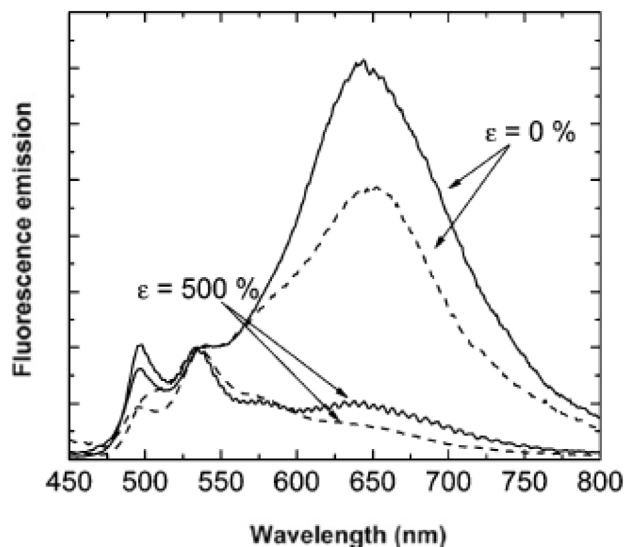
FIGURE 10 Fluorescence spectra of PE films containing OPV1 (solid lines) or OPV2 (dashed lines) at 0% and 500% strain. Reproduced with permission. 22 Copyright 2007, American Chemical Society
