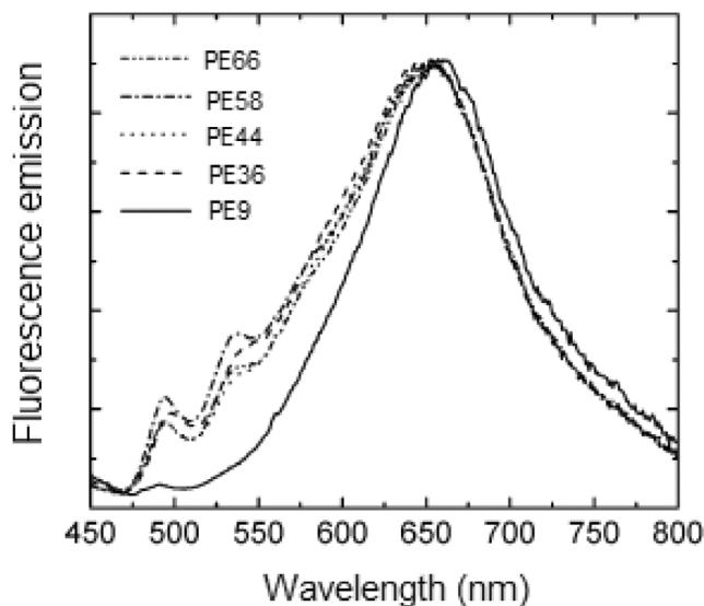
FIGURE 20 Fluorescence spectra of PE/OPV2 blends with different polymer crystallinities. Adapted figure with permission. 22 Copyright 2007, American Chemical Society
