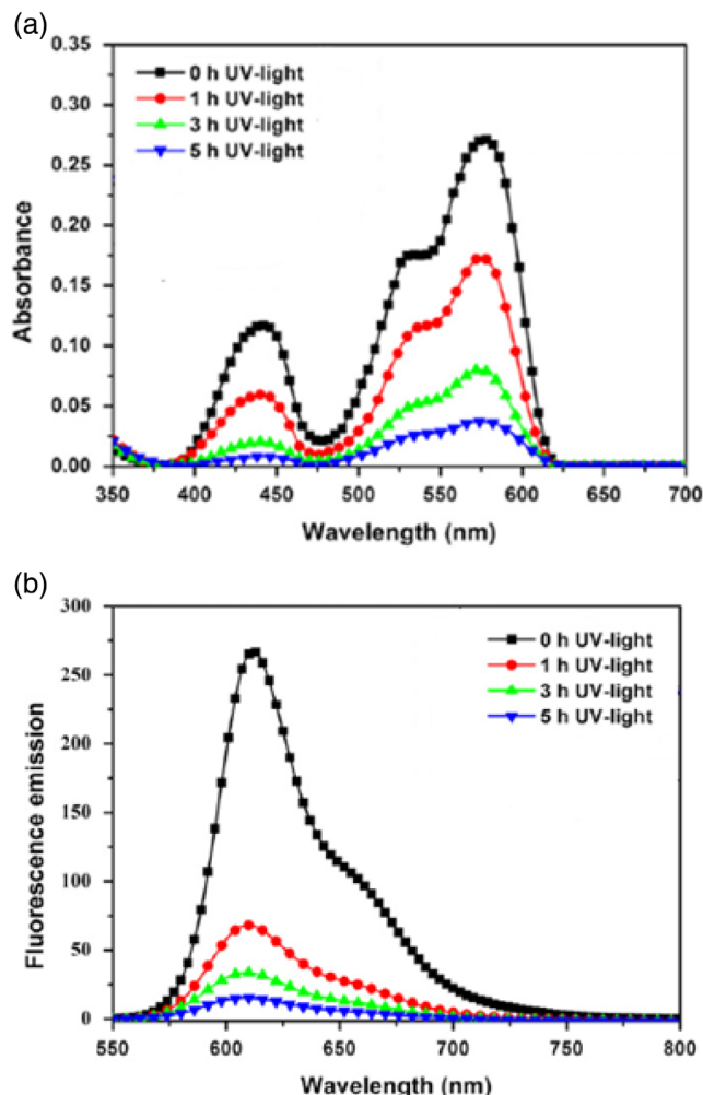
FIGURE 3 Absorption (a) and fluorescence (b) spectra of PMMA/Pery1 blends after 1, 3, and 5 h of UV light exposure. Reproduced with permission. 17 Copyright 2013, Elsevier [Color figure can be viewed at wileyonlinelibrary.com ]
