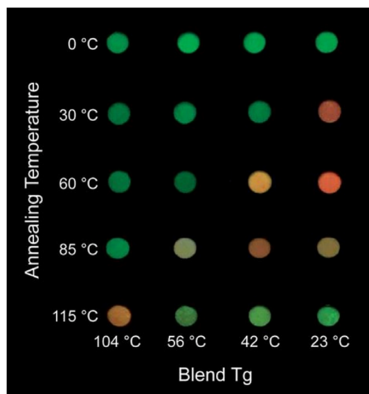
FIGURE 16 Images of quenched PAMx blends annealed for at least 15 h at various temperatures. Reproduced with permission. 32 Copyright 2007, Wiley-VCH [Color figure can be viewed at wileyonlinelibrary.com ]
