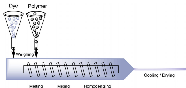
FIGURE 9 Polymer/dye blend preparation using a melt-extrusion process. [Color figure can be viewed at wileyonlinelibrary.com ]
