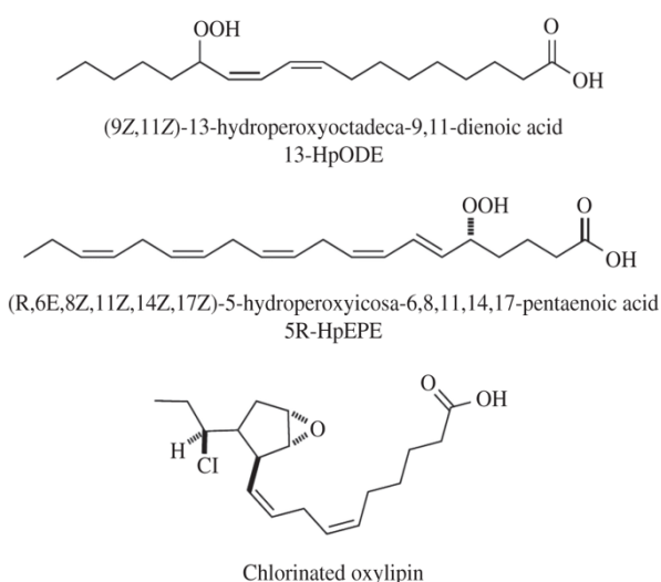
Figure 4: Oxylipins in algae. 13-HpODE is identified in Chondrus crispus (Rhodophyta, Gigartinales ) (Fontana et al., 2007); 5R-HpEPE in Skeletonema marinoi (Bacillariophyta, Thalassiosirales ) (D'Ippolito et al., 2005) and the chlorinated oxylipin in Egregia menziesii (Ochrophyta, Laminariales ) (Dembitsky & Srebnik, 2002).
