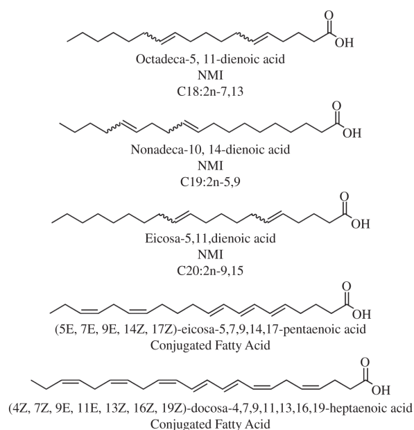
Figure 2: Chemical structure of non-methylene-interrupted fatty acids (NMI) and conjugated fatty acid identified in algae. C18:2n-7,13 is identified in Cladophora rupestris (Chlorophyta, Chladophorales ) (Ratnayake & Ackman, 1979); C19:2n-5,9 in Grateloupia turuturu (Rhodophyta, Halymeniales ) (Kendel et al., 2013) and C20:2n-9,15 in Sargassum species (Ochrophyta, Fucales ) (Khotimchenko, 1991). The conjugated fatty acid (5E,7E,9E, 14Z, 17Z)-eicosa-5,7,9,14,17-pentaenoic acid is found in Acanthophora spicifera (Rhodophyta, Ceramiales ) (Bhaskar, Kinami, et al., 2004) and (4Z, 7Z, 9E, 11E, 13Z, 16Z, 19Z)-docosa-4,7,9,11,13,16,19-heptaenoic acid in Anadyomene stellata (Chlorophyta, Chladophorales ) (Mikhailova et al., 1995).
