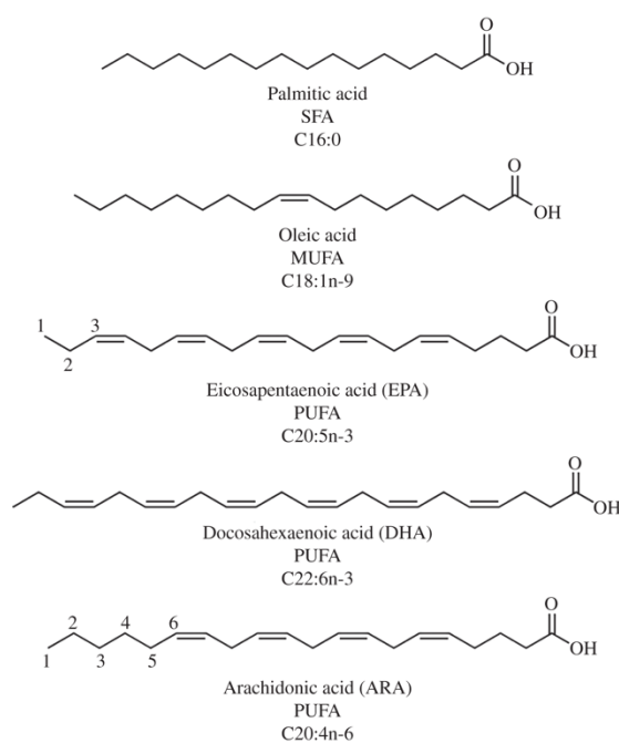
Figure 1: Chemical structure examples of Saturated Fatty Acid (SFA), Monounsaturated Fatty Acid (MUFA) and Polyunsaturated Fatty Acids (PUFA).
