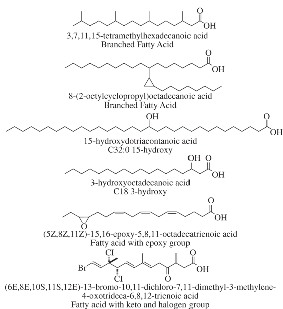
Figure 3: Branched and functionalized fatty acids. 3,7,11,15-tetramethylhexadecanoic acid is identified in Heterococcus fuornensis (Ochrophyta, Tribonematales ) (Lang et al., 2011); 8-(2-octylcyclopropyl)octadecanoic acid in Chlamydomonas zebra (Chlorophyta, Chlamydomonadales ) (Lang et al., 2011), 15-hydroxydotriacontanoic acid in Nannochloropsis sp. (Ochrophyta, Eustigmatales ) (Gelin et al., 1997); 3-hydroxyoctadecanoic acid in Solieria chordalis (Rhodophyta, Gigartinales ) (Kendel et al., 2015); (5Z,8Z,11Z)-15,16-epoxy-5,8,11-octadecatrienoic acid in Chlamydomyxa montana (Ochrophyta, Chlamydomyxales ) (Lang et al., 2011) and (6E,8E,10S,11S,12E)-13-bromo-10,11-dichloro-7,11-dimethyl-3-methylene-4-oxotrideca-6,8,12-trienoic acid in Plocamium cartilagineum (Rhodophyta, Plocamiales ) (Dembitsky & Srebnik, 2002).
