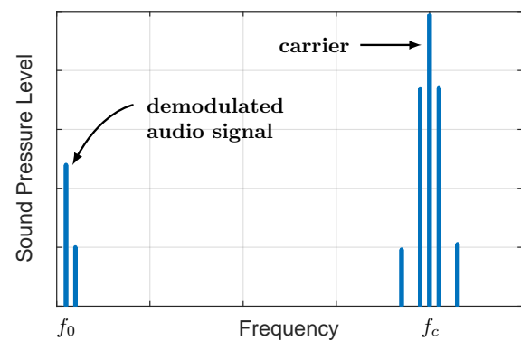
(b) spectrum of the of the resulting analogue signal (b)
