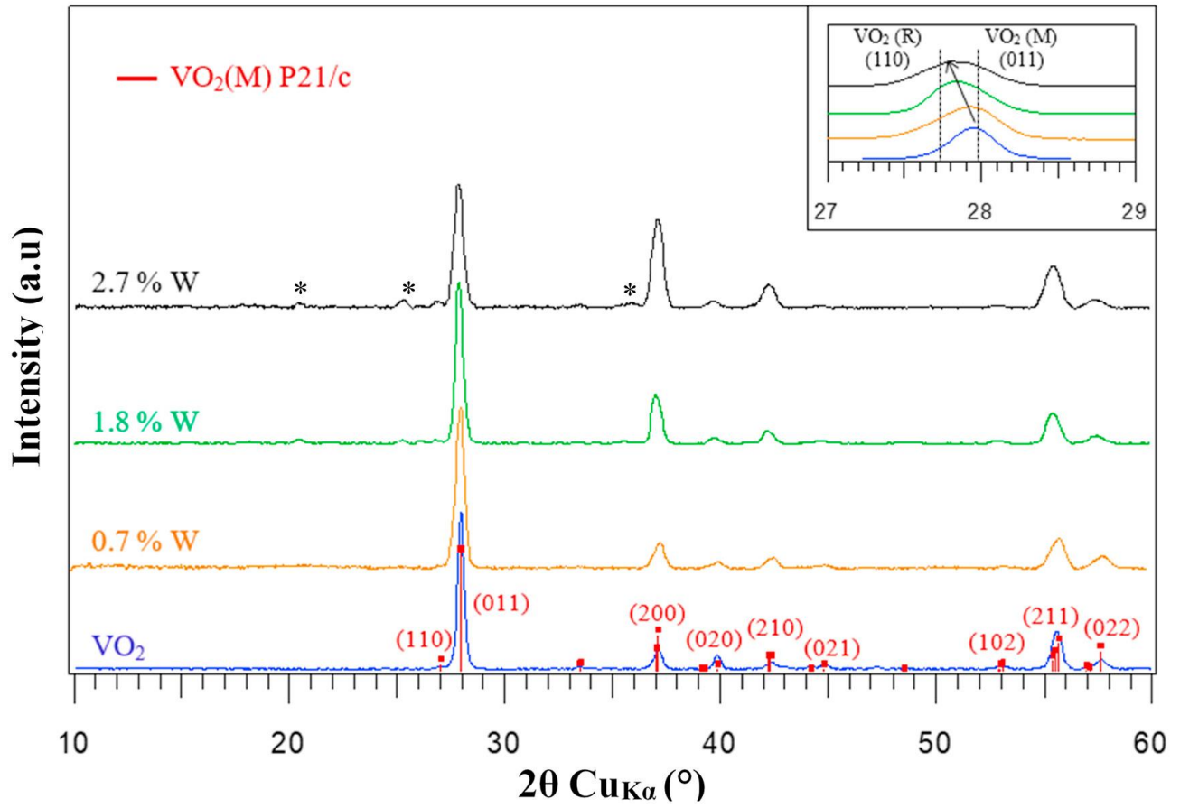
Fig. 2. X-ray Diffraction pattern from \theta - 2\theta scans of V_{1-x}W_xO_{2\pm\delta} thin films deposited by PDCMS and magnification of the 27–29 2\theta region corresponding to the VO_2(M) (011) and VO_2(R) (110), * impurity phase tentatively assigned as V_6O_{13} .
