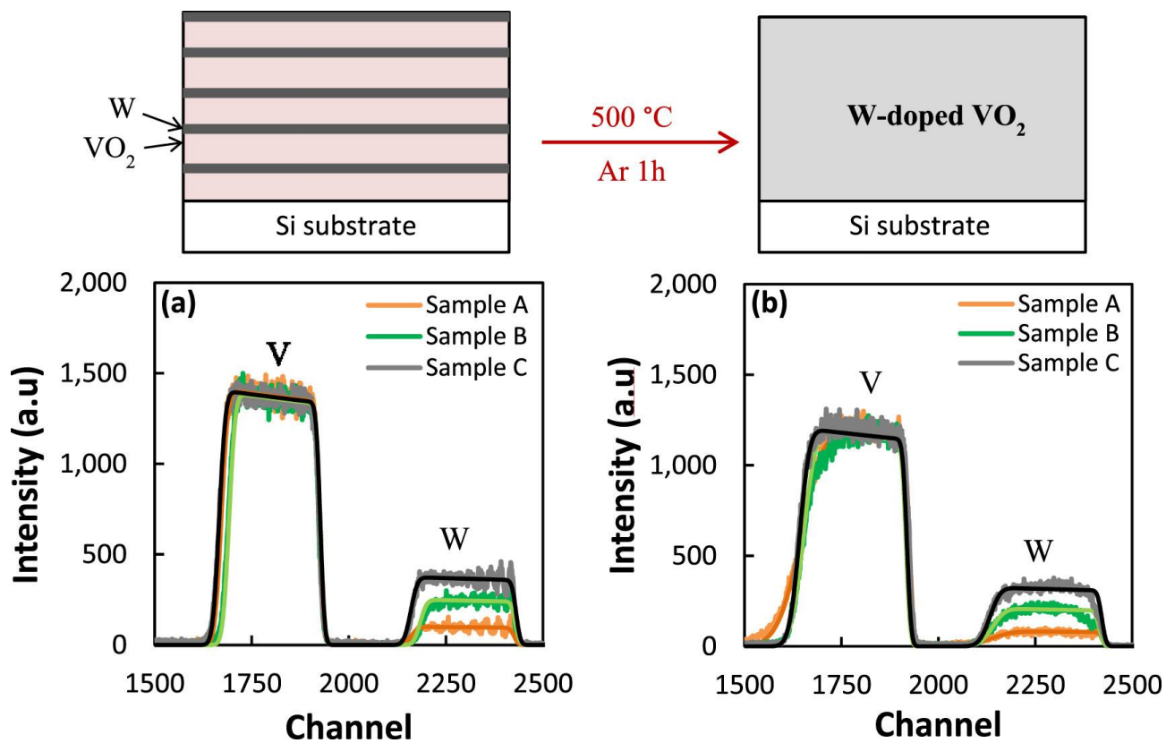
Fig. 1. RBS spectra of the W-doped VO 2 thin films on Si substrate before thermal annealing (a) and after thermal annealing at 500 °C in Ar for 1h (b).
