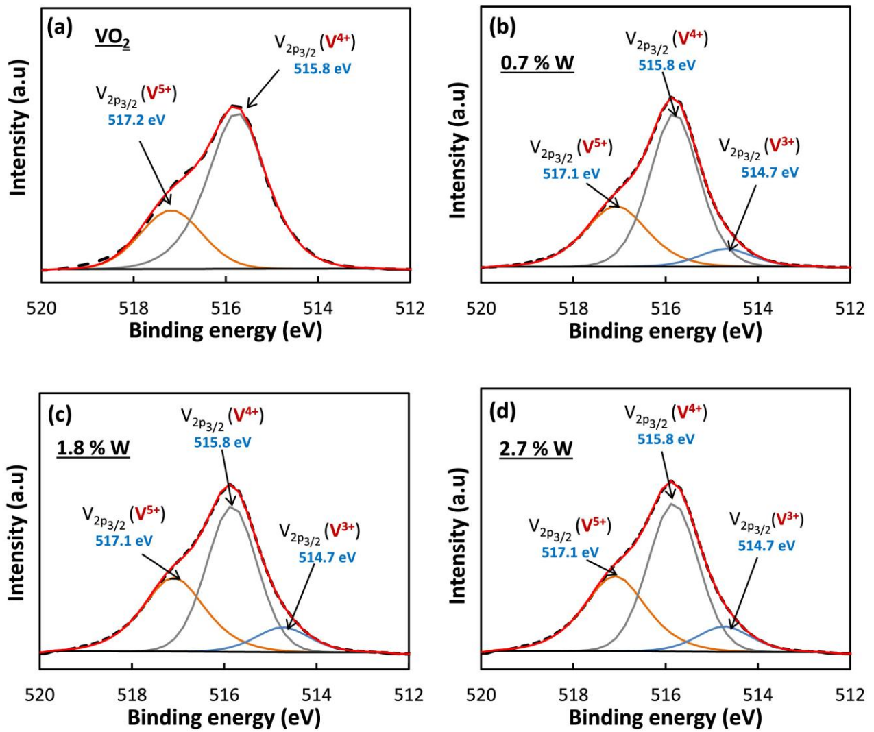
Fig. 4. The core level spectra of V_{2p} of VO_2 (a) 0.7% W (b) 1.8% W (c) and 2.7% W (d) in V_{1-x}W_xO_{2+\delta} films.
