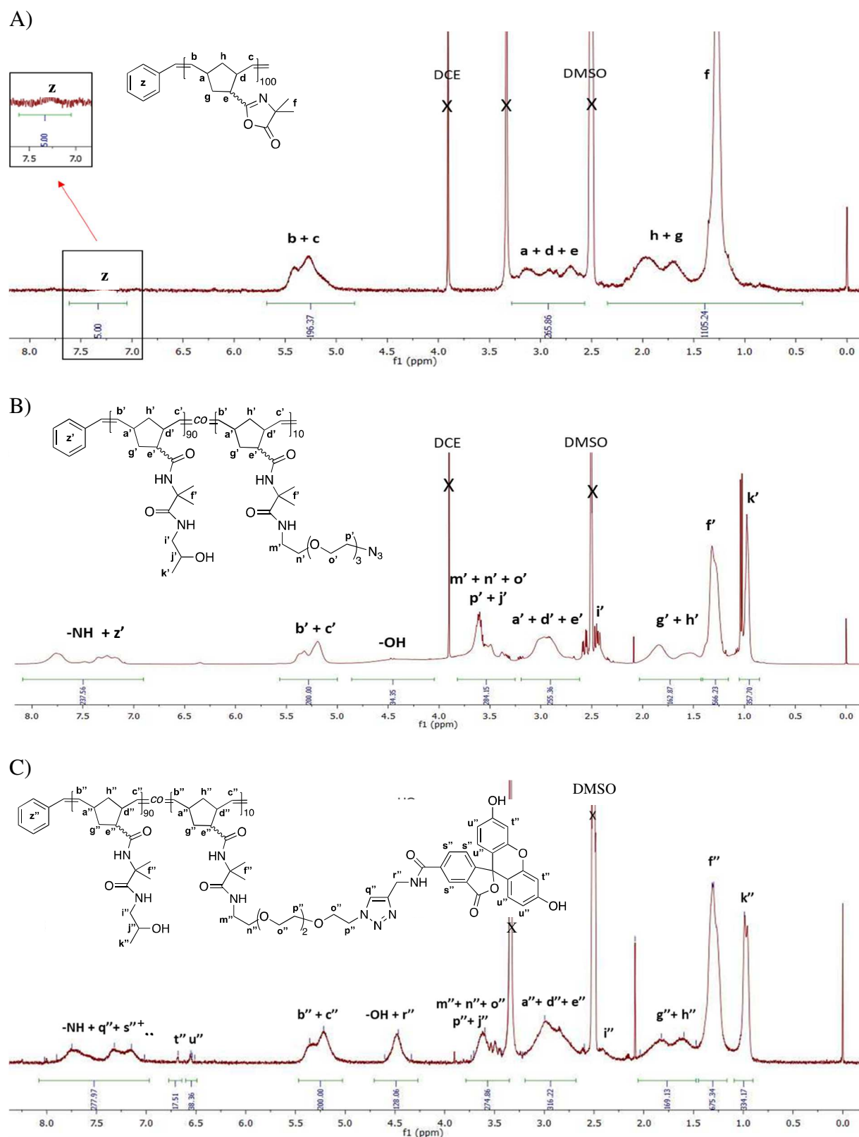
Fig. 1. ^1\text{H} NMR spectra of (A) PNBAzl (Table 1, run 2), (B) (m\text{-PNBAzl-OH})_{90}\text{-co-}(m\text{-PNBAzl-N}_3)_{10} and (C) (m\text{-PNBAzl-OH})_{90}\text{-co-}(m\text{-PNBAzl-fluorescein})_{10} ; solvent: \text{DMSO-}d_6 .
