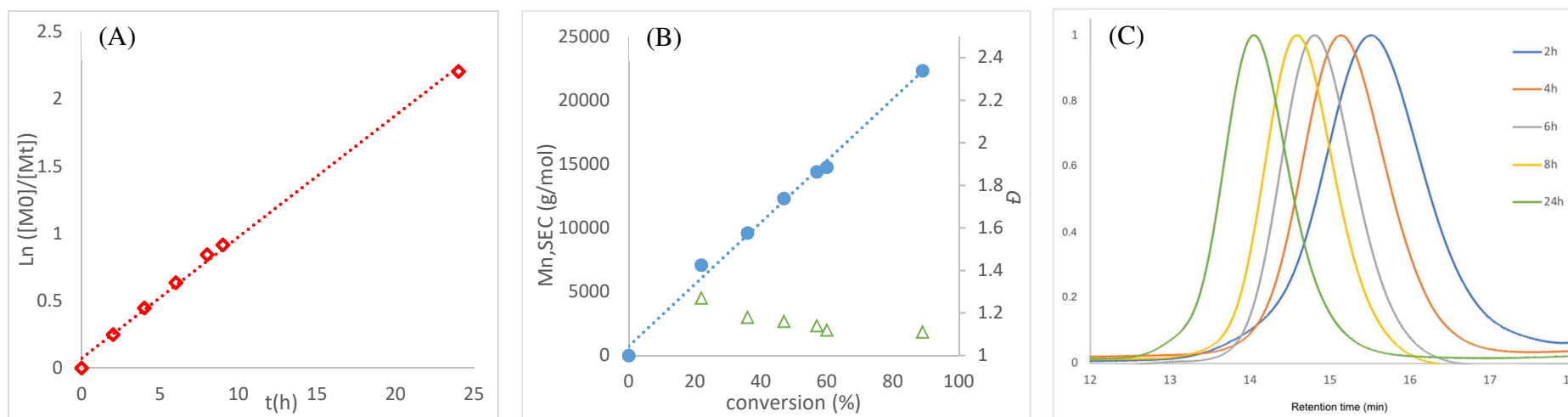
Fig. 3. (A) Kinetic plot - \ln([M]_t/[M]_0) as a function of reaction time (B) \overline{M}_{n,SEC} and D versus conversion of NBAzl , and (C) SEC traces of crude polymers at different conversions of monomer for the ROMP of NBAzl using G3' as the initiator with an initial monomer concentration of 0.05 mol.L -1 and a [M]_0/[I]_0 ratio of 100 at 70 °C in DCE (THF eluent; RI detector).
