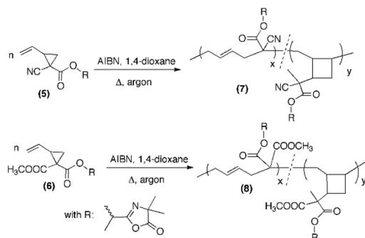
Scheme 2 Free-radical polymerization of ( 5 ) and ( 6 ) using AIBN as an initiator in 1,4-dioxane.
