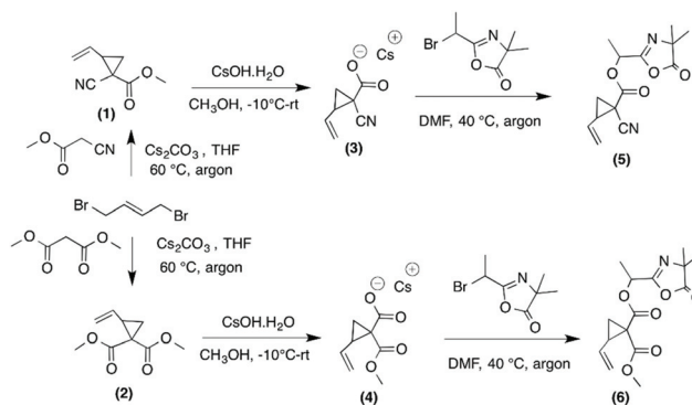
Scheme 1 Synthesis of azlactone-functionalized vinylcyclopropanes (5) and (6).
