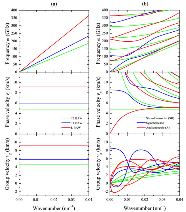
Fig. 1. Dispersion relation of acoustic phonons propagating in (a) [110] of bulk silicon and (b) [110] of 250 nm thick Si (001) membrane.
