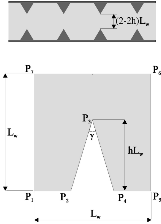
FIG. 2. Geometry of two-dimensional pore channel (top) and of the periodic cell (bottom).
