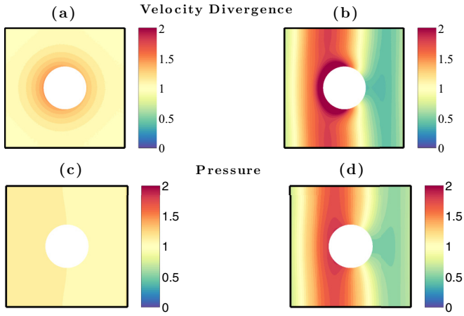
FIG. 4. Field distribution for velocity divergence (a), (b) and pressure (c), (d). Normalized velocity divergence (a), and pressure (c), at normalized frequency k_0 L / \pi = 0.1 in the domain of validity of the local theory, where \lambda \gg L . Normalized velocity divergence (b), and pressure (d), at normalized frequency k_0 L / \pi = 1 in Bragg's regime.
