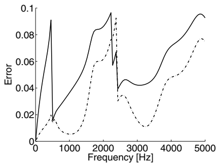
Figure 6. Error with a truncation criterion on the residual \varepsilon_1 = \varepsilon_2 = 0.1 . Solid: Error relative to the left substructure; Dash-dot: Error relative to the right substructure.
