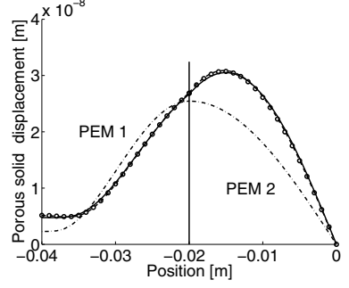
Figure 2. Solid displacement of the two porous structures. Solid: analytical solution; Dash-dot: DMT; Dash: ICMT; Circles: FICMT.
