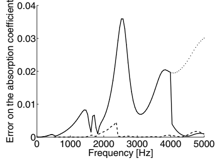
Figure 9. Error on the absorption coefficient versus frequency. Dash: \varepsilon = 0.1 ; Solid: \varepsilon = 0.5 ; Dot: \varepsilon = 2 .
