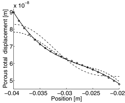
Figure 4. Total displacement of the two porous structures, detail near the excitation. Solid: analytical solution; Dash-dot: DMT; Dash: ICMT; Circles: FICMT.
