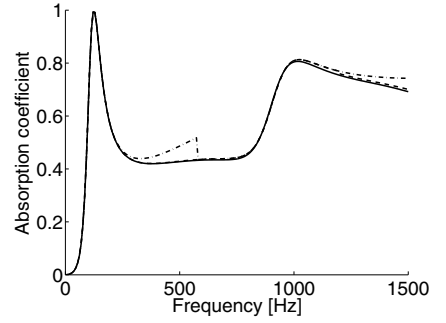
Figure 11. Absorption coefficient versus frequency. Solid: Exact solution; Dash-dot: \epsilon = 0.4 ; Dash: \epsilon = 0.2 .
