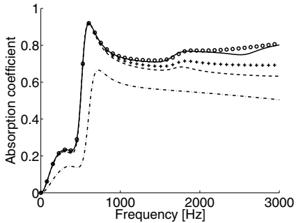
Figure 5. Absorption coefficient versus frequency for 1 mode in each porous substructure. Solid: analytical solution; Dash-dot: DMT; Dash: ICMT; Circles: FICMT; Plus: FICMT under assumption that the contribution of the attachment mode associated to the force is 1.
