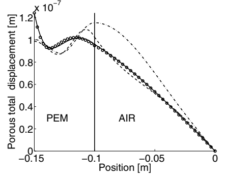
Figure 10. Total displacement of the porous structure and air displacement. Solid: analytical solution; Dash-dot: DMT; Dash: ICMT; Circles: FICMT.
