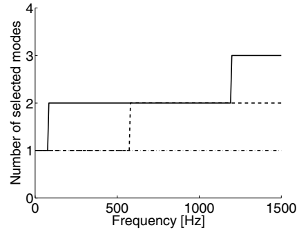
Figure 12. Number of selected modes versus frequency. Solid: Modes of the porous substructure \epsilon = 0.2 ; Dash-dot: Modes of the air substructure \epsilon = 0.2 ; Dash: Modes of the porous substructure \epsilon = 0.4 .
