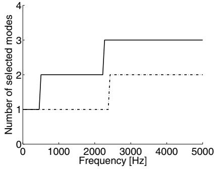
Figure 7. Number of selected modes versus frequency. Solid: Modes of the left substructure \varepsilon = 0.1 ; Dash-dot: Modes of the right substructure \varepsilon = 0.1 .
