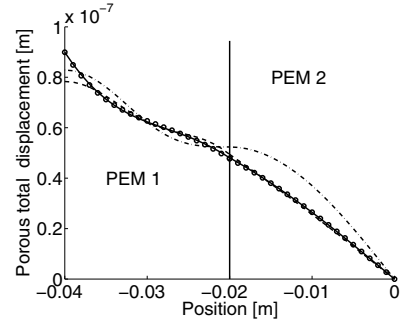
Figure 3. Total displacement of the two porous structures. Solid: analytical solution; Dash-dot: DMT; Dash: ICMT; Circles: FICMT.
