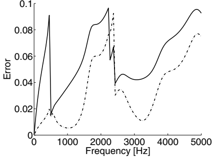
Figure 6. Error with a truncation criterion on the residual \varepsilon_1 = \varepsilon_2 = 0.1 . Solid: Error relative to the left substructure; Dash-dot: Error relative to the right substructure.
