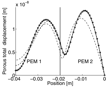
Figure 8. Total displacement at 2300 Hz. Solid: Analytical solution; Dash-dot: Solution with (2;1) modes; Dash: Solution with (2;2) modes; Circles: Solution with (3;2) modes.
