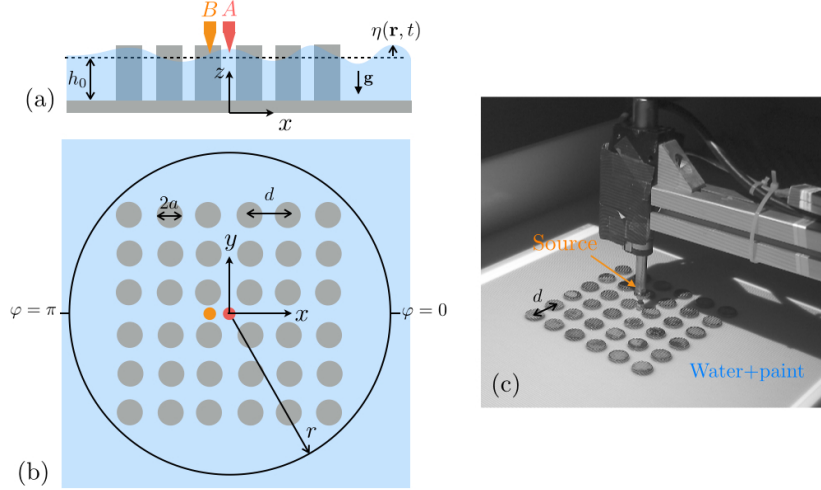
Figure 1. Geometry of the 6 \times 6 square lattice (a) side view and (b) top view, (c) experimental set-up; A and B show the two source positions inside the array.
