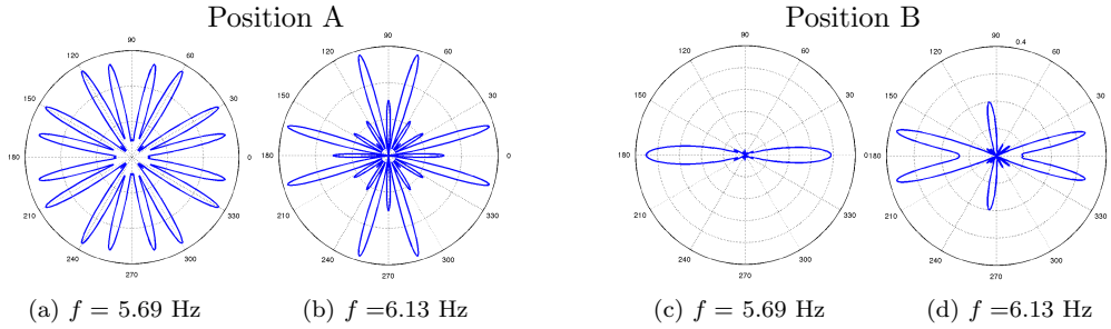
Figure 2. Directional emission, f_{\text{tot}}(\varphi) in Eq. (4), of the source embedded in the lattice (a)-(b) with the point source at A and (c)-(d) with the point source at B. Frequencies are (a) and (c) at f = f_0 = 5.69 Hz (band edge frequency), (b) and (d) at f = 6.13 Hz. Corresponding wavefields are shown in Figs. 6(c) and (f) for position A and 8(c) and (f) for position B.
