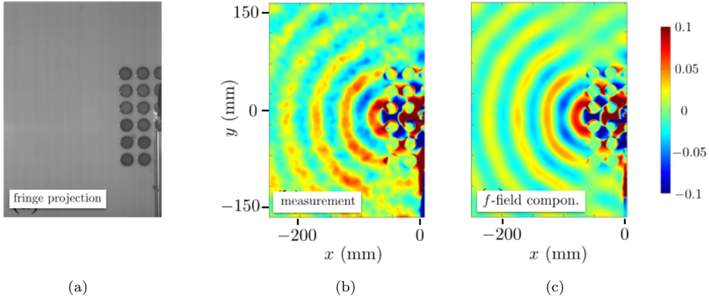
Figure 4. (a) Picture corresponding to the measurement domain, as recorded by the camera, (b) Typical instantaneous measured field using FTP (the colorbar is in mm, for the values of \eta(\mathbf{r}, t) ), (c) Real part of the complex field corresponding to the linear field \eta_1(\mathbf{r}) , Eqs. (7)-(8)
