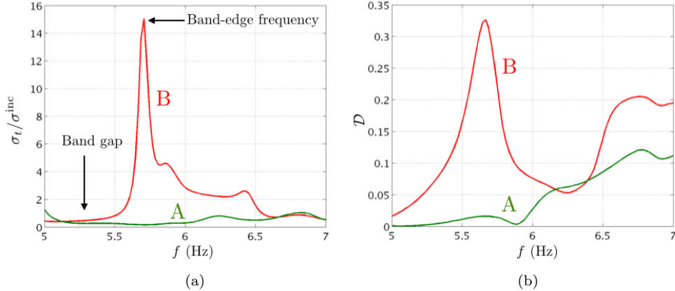
Figure 3. (a) Total cross section \sigma_t/\sigma^{\text{inc}} as a function of the frequency. (b) Directivity \mathcal{D} , reflecting the energy transported by the beams emerging along the x -direction (with angular aperture \Delta\varphi = 8^\circ ).
