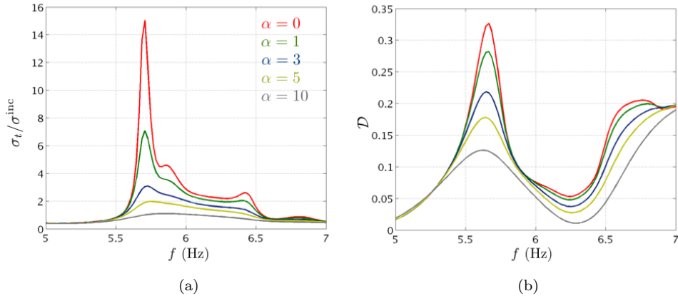
Figure 9. (a) Normalized total cross section \sigma_t/\sigma^{\text{inc}} and (b) factor of directivity \mathcal{D} as a function of the frequency f for various attenuation factors \alpha (in \text{m}^{-1} ).
