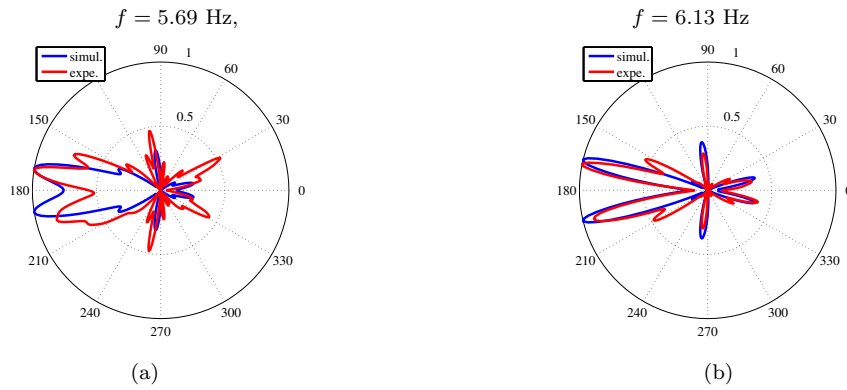
Figure 8. Point source at position B. Same representation as in Figure 6.
