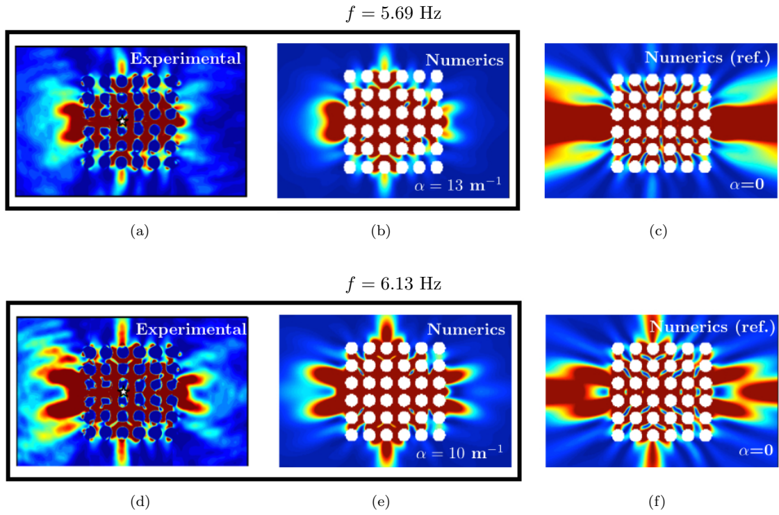
Figure 7. Point source at position B. Same representation as in Figure 5.
