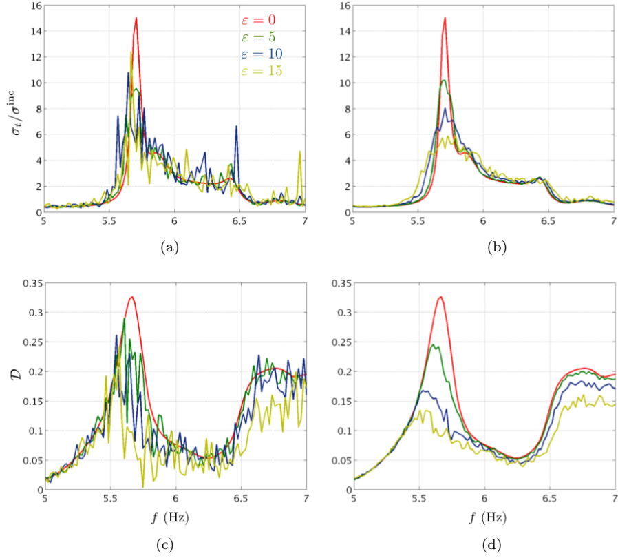
Figure 10. Influence of the disorder on the directional emission. (a-b) Total directivity function \sigma_t/\sigma^{\text{inc}} and (c-d) directivity parameter \mathcal{D} . (a) and (c) correspond to a typical response of the structure for one realization of the disordered structure (with amplitude of disorder measured by \varepsilon ); (b) and (d) correspond to the response of the periodic-on-average structure (here 40 averages have been performed).
