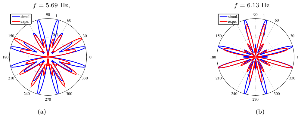
Figure 6. Point source at position A. Total directivity functions f_{\text{tot}}(\varphi) , Eq. (4), measured at r = 120 mm. Red curves, experimental, deduced from the measurement of |\eta(\mathbf{r})|^2 . Blue curves, numerical results using MST and with attenuation (a) \alpha=13 \text{ m}^{-1} and (b) \alpha=10 \text{ m}^{-1} .
