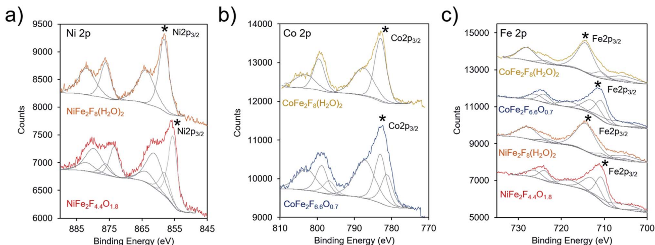
Fig. 5 XPS spectra of the (oxy)fluorides and oxyfluorides. The (a) Ni 2p 3/2 , (b) Co 2p 3/2 and (c) Fe 2p 3/2 were acquired and spectra subsequently fit to (grey traces) compare with database data of F-free oxides. The 2p 3/2 peaks discussed are denoted with a *.
