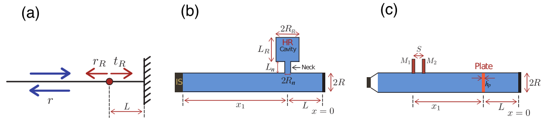
Figure 1. (a) Asymmetric Fabry-Pérot resonator made of a resonant element (red point) and a rigid backing at distance L from the resonator. (b,c) respectively show the SRS and the SMRS set-ups. In the set-up (b) an Impedance Sensor (IS) 25 is used for the measurements. In (c) two microphones placed before the sample are used to experimentally characterize the system 29 .
