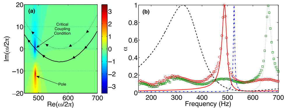
Figure 2. SRS configuration. (a) Represents the complex frequency map of \log |r| for the SRS with L_R = 8.3 cm. Black dashed (continuous) line represents the trajectory of the zero of |r| for the lossless (lossy) case in the complex plane increasing L_R [sense of the increasing shown by arrows over the lines]. (b) Red continuous and green dotted lines (open red circles and open green squares) represent the absorption coefficient \alpha for the configurations (L_R, f_{CC}) = (8.3 \text{ cm}, 484.5 \text{ Hz}) and (L_R, f_{CC}) = (3.9 \text{ cm}, 647 \text{ Hz}) . Blue dash-dotted line represents the absorption coefficient for the configuration (L_R, f_{CC}) = (7 \text{ cm}, 526 \text{ Hz}) with half inherent losses of the experimental case. Black dashed line represents the absorption coefficient for the configuration (L_R, f_{CC}) = (16 \text{ cm}, 330 \text{ Hz}) with 20 times the inherent losses of the experimental case.
