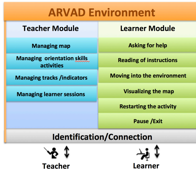
Fig. 6. ARVAD Software Architecture
