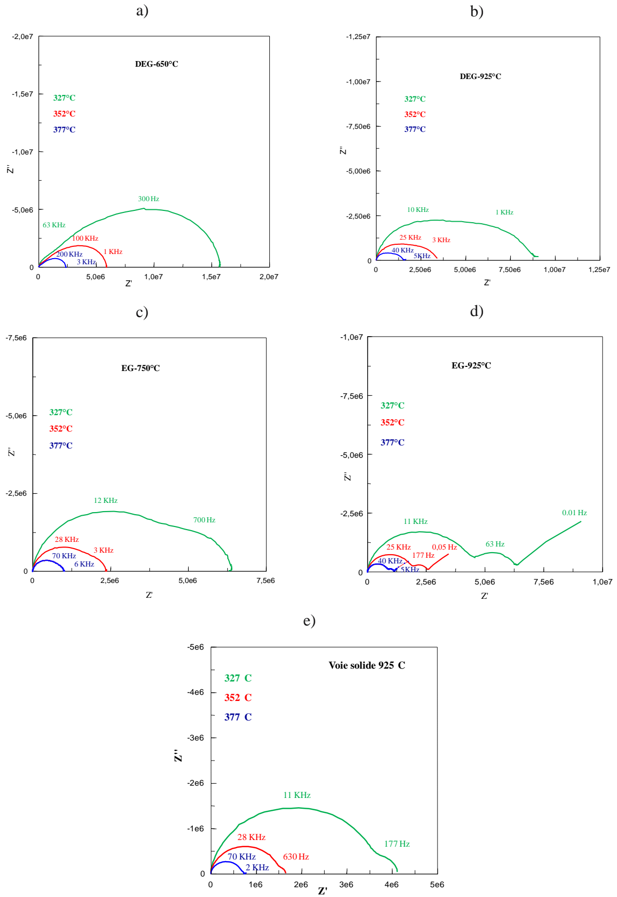
Figure 17: Complex impedance diagram recorded at 327, 352 and 377 °C for pellets made of powders synthesized with DEG and sintered at 650 (a) or 925 °C (b), and with EG ( u = 3 ) and
