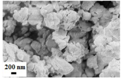
Figure 10: SEM images of the precipitate synthesized with DEG or EG ( u = 3 ) and hydrolysis ratio h = 2 , then heat treated at 600°C for 5min.
