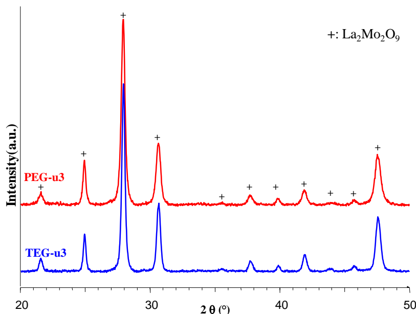
Figure 4: XRD diagrams of precipitates synthesized with PEG ( u = 3 ) or TEG ( u = 3 ) and heat treated at 600°C for 5min.
