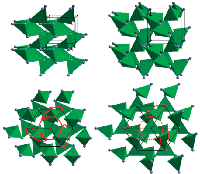
Figure 6. Folded (left, exaggerated) and unfolded (right) anti-framework as viewed along two directions of the \beta -La 2 Mo 2 O 9 type structure: along the tunnels parallel to the cubic cell axis (upper) and along the 3-fold axis (lower). The rotation of [O1La 3 Mo] anti-tetrahedral units is outlined.
