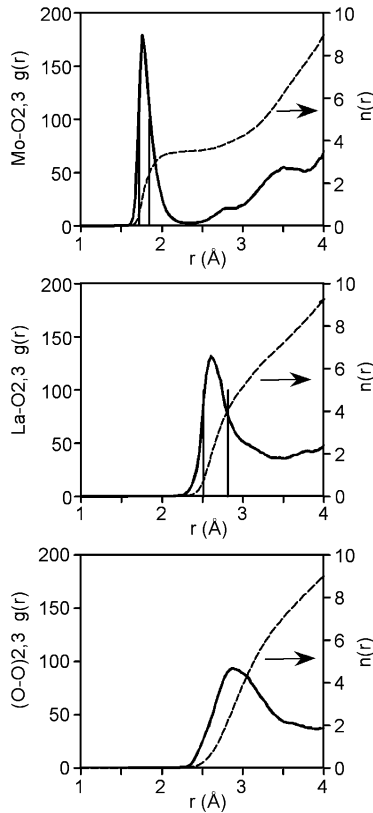
Figure 11. Radial distribution function g_{ij}(r) and coordination number distribution n_{ij}(r) versus the interionic distance r in the cation–anion (Mo–O 2,3 and La–O 2,3 ) and anion–anion (O 2,3 –O 2,3 ) pairs, after molecular dynamics relaxation at 943 K. For full cationic coordination numbers, one and three O1 extra neighbors should be added to Mo and La polyhedra, respectively. Vertical lines correspond to the crystal structure interatomic distances (from ref 18).
