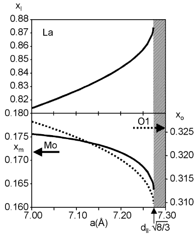
Figure 5. Position of the atoms of rigid [O1La 3 Mo] anti-tetrahedral units in the crystal cell as a function of the cubic cell parameter (from interatomic distances measured in \beta -La 2 Mo 2 O 9 at 670 °C: 18 d_{II} = 4.454 Å, d_{Im} = 3.703 Å, d_{mo} = 1.839 Å).
