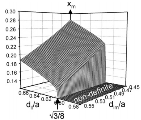
Figure 4. Molybdenum atomic coordinate x_m as a function of d_{\parallel}/a and d_{\text{lm}}/a in a semirigid [\text{OLaMo}] framework.
