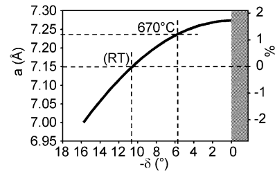
Figure 7. Calculated cubic cell parameter as a function of the \delta rotation angle of rigid [O1La 3 Mo] anti-tetrahedral units (with imposed geometry d_{II} = 4.454 Å, d_{Im} = 3.703 Å, d_{mo} = 1.839 Å). The dashed lines indicate the cell parameter and rotation angle of \beta -La 2 Mo 2 O 9 at 670 °C (from crystal structure data, ref 18) and their approximation in a pseudo-cubic cell at room temperature.
