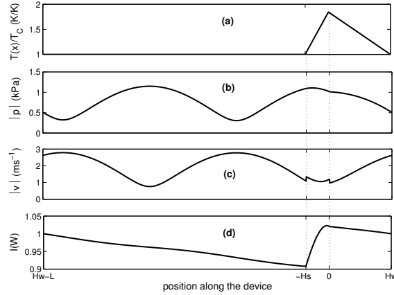
Figure 3: Distribution of the acoustic pressure |\tilde{p}(x)| (b), acoustic velocity |\tilde{v}(x)| (c), and acoustic intensity I = (1/2)\text{Re}(\tilde{p}\tilde{v}^*) (d) in the whole device, at threshold for the case of the linear temperature distribution profile (a).
