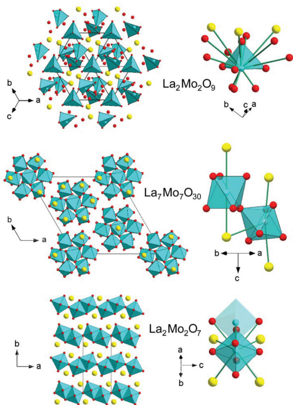
Fig. 2 Global configuration (left) and local arrangement around Mo (right) in the structures of crystallized \beta - \text{La}_2\text{Mo}_2\text{O}_9 (upper), \text{La}_7\text{Mo}_7\text{O}_{30} (middle) and \text{La}_2\text{Mo}_2\text{O}_7 (lower). Mo coordination polyhedra are in blue as well as Mo ions, \text{La}^{3+} ions are in yellow and \text{O}^{2-} ions in red. Note that Mo coordination polyhedra are isolated in \text{La}_2\text{Mo}_2\text{O}_9 , corner-sharing in \text{La}_7\text{Mo}_7\text{O}_{30} , and edge-sharing in \text{La}_2\text{Mo}_2\text{O}_7 .
