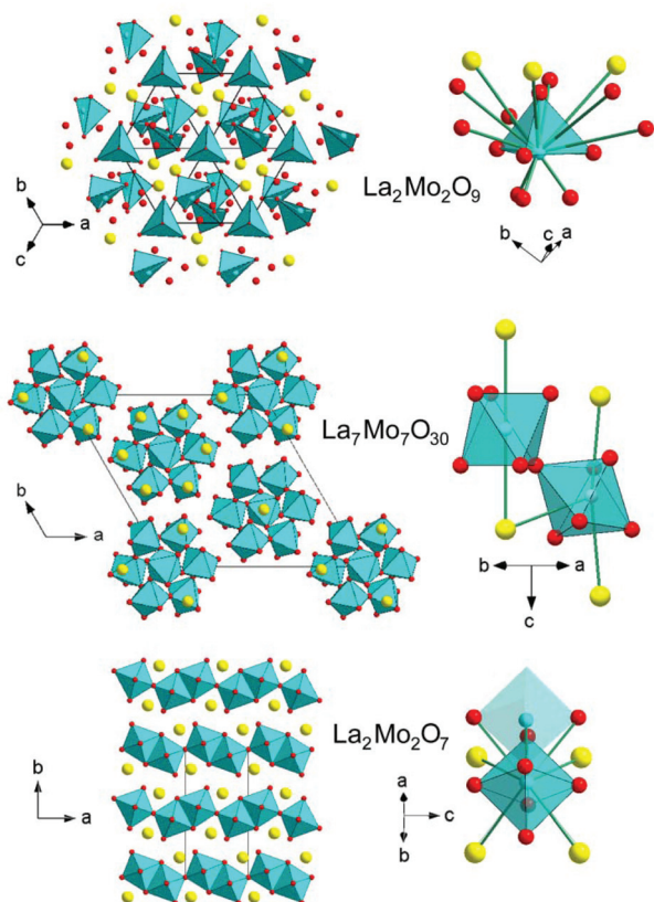
Fig. 2 Global configuration (left) and local arrangement around Mo (right) in the structures of crystallized \beta\text{-La}_2\text{Mo}_2\text{O}_9 (upper), \text{La}_7\text{Mo}_7\text{O}_{30} (middle) and \text{La}_2\text{Mo}_2\text{O}_7 (lower). Mo coordination polyhedra are in blue as well as Mo ions, \text{La}^{3+} ions are in yellow and \text{O}^{2-} ions in red. Note that Mo coordination polyhedra are isolated in \beta\text{-La}_2\text{Mo}_2\text{O}_9 , corner-sharing in \text{La}_7\text{Mo}_7\text{O}_{30} , and edge-sharing in \text{La}_2\text{Mo}_2\text{O}_7 .
