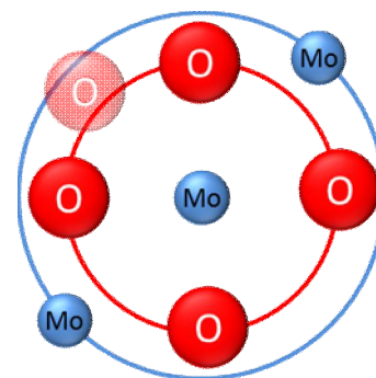
Figure 14: Scheme of coordination shells around Mo in amorphous \text{La}_2\text{Mo}_2\text{O}_{6.72} with models B or E of SSpaths EXAFS analysis.
