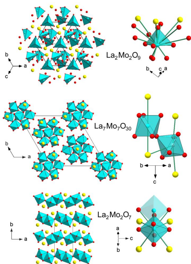
Figure 2: Global configuration (left) and local arrangement around Mo (right) in the structures of crystallized \beta\text{-La}_2\text{Mo}_2\text{O}_9 (upper), \text{La}_7\text{Mo}_7\text{O}_{30} (middle) and \text{La}_2\text{Mo}_2\text{O}_7 (lower). Mo coordination polyhedra are in blue as well as Mo ions, \text{La}^{3+} ions are in yellow and \text{O}^{2-} ions in red. Note that Mo coordination polyhedra are isolated in \text{La}_2\text{Mo}_2\text{O}_9 , corner-sharing in \text{La}_7\text{Mo}_7\text{O}_{30} , and edge-sharing in \text{La}_2\text{Mo}_2\text{O}_7 .
