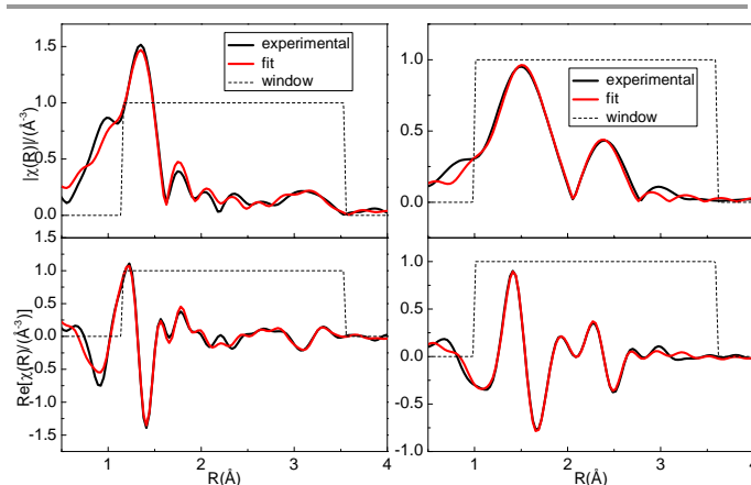
Figure 6: Fourier Transform of EXAFS oscillations at the molybdenum K-edge for \text{La}_2\text{Mo}_2\text{O}_9 (left) and \text{La}_2\text{Mo}_2\text{O}_{6.72} (right): modulus (upper) and real part (lower). Red lines show the fit of EXAFS data with 6 coordination shells around Mo.
