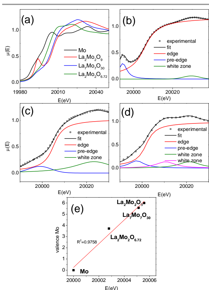
Figure 4: (a) comparison of normalized molybdenum K-edge XANES data collected at room temperature on different molybdates and metallic Mo; fit of the edge, pre-edge and white zone for XANES analysis of: (b) \text{La}_2\text{Mo}_2\text{O}_9 , (c) \text{La}_7\text{Mo}_7\text{O}_{30} and (d) amorphous \text{La}_2\text{Mo}_2\text{O}_{6.72} ; (e) valence of Mo as a function of the energy of the edge E_0 .
