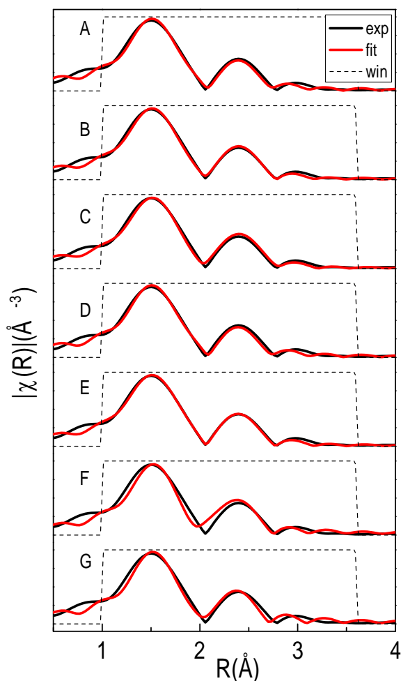
Figure 13: Modulus of Fourier Transform of EXAFS oscillations at the molybdenum K-edge for amorphous \text{La}_2\text{Mo}_2\text{O}_{6.72} with the fits based on seven different arrangements generated by SSpaths.
