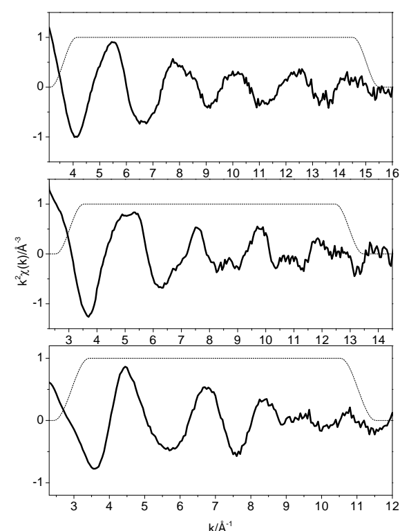
Figure 5: EXAFS signal multiplied by k^2 and selected range for FT for: (a) crystalline \text{La}_2\text{Mo}_2\text{O}_9 , (b) crystalline \text{La}_7\text{Mo}_7\text{O}_{30} and (c) amorphous \text{La}_2\text{Mo}_2\text{O}_{6.72} .
