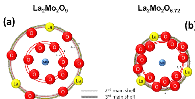
Figure 7: Schemes of coordination shells around Mo, obtained from EXAFS analysis in: (a) crystalline La 2 Mo 2 O 9 ; (b) amorphous La 2 Mo 2 O 6.72 within a La 2 Mo 2 O 9 type model of local order.
