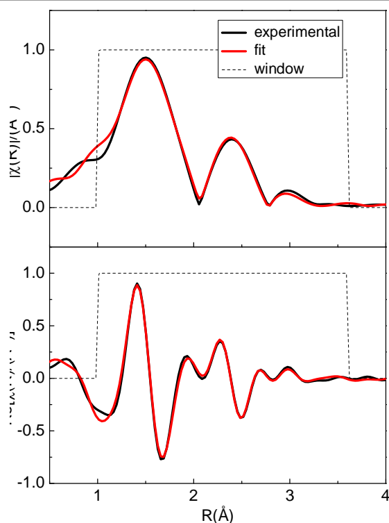
Figure 9: Fourier Transform of EXAFS oscillations at the molybdenum K-edge for amorphous \text{La}_2\text{Mo}_2\text{O}_{6.72} : modulus (upper) and real part (lower). Red lines show the fit of EXAFS data with 7 coordination shells around Mo in \text{La}_2\text{Mo}_2\text{O}_7 .
