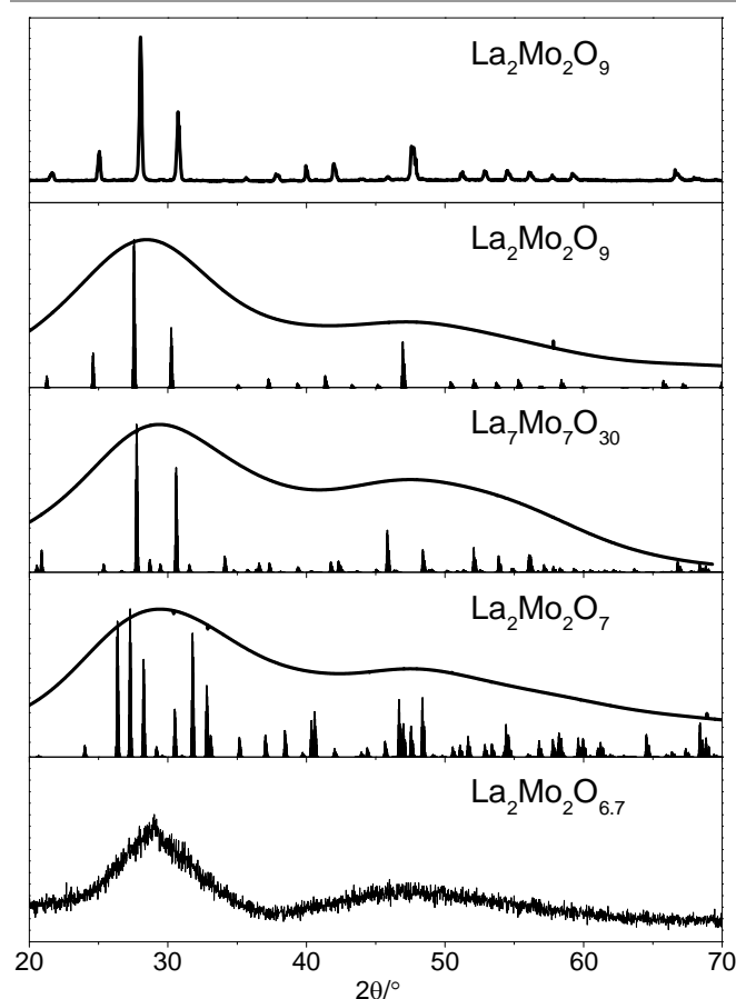
Figure 3: XRD pattern of \text{La}_2\text{Mo}_2\text{O}_9 (top) and amorphous \text{La}_2\text{Mo}_2\text{O}_{6.72} (bottom) with in between simulated XRD patterns of \text{La}_2\text{Mo}_2\text{O}_9 , \text{La}_7\text{Mo}_7\text{O}_{30} and \text{La}_2\text{Mo}_2\text{O}_7 assuming large (narrow peaks) and very small crystallite sizes (broad envelopes) from PDF4+ database software 28 .
