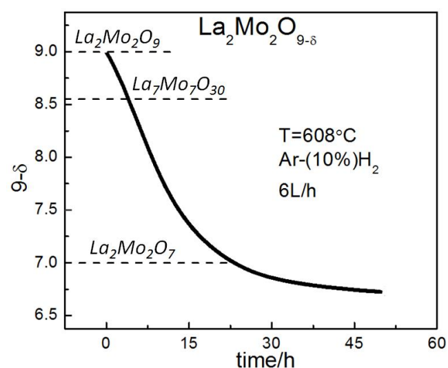
Figure 1: Thermogravimetric curve of the reduction of a \text{La}_2\text{Mo}_2\text{O}_9 powder at 608 °C in diluted \text{H}_2 .
