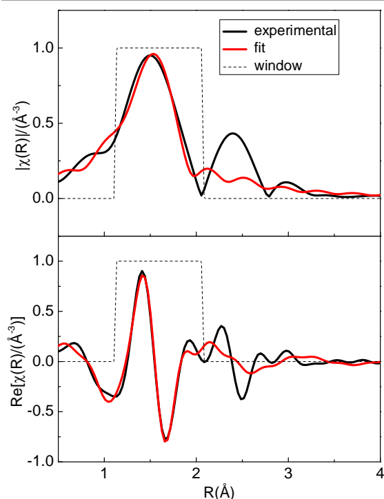
Figure 12: Fourier Transform of EXAFS oscillations at the molybdenum K-edge for amorphous \text{La}_2\text{Mo}_2\text{O}_{6.72} : modulus (upper) and real part (lower). Red lines show the first O shell fit.
