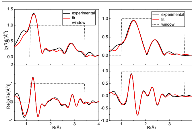
Figure 8: Fourier Transform of EXAFS oscillations at the molybdenum K-edge for \text{La}_7\text{Mo}_7\text{O}_{30} (left) and \text{La}_2\text{Mo}_2\text{O}_{6.72} (right): modulus (upper) and real part (lower). Red lines show the fit of EXAFS data with 8 coordination shells around two Mo sites.
