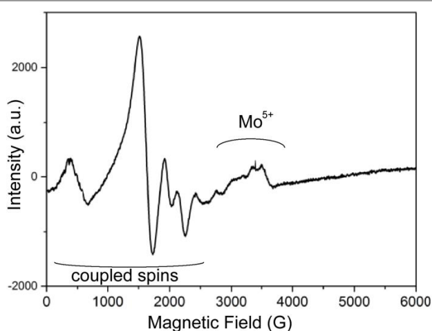
Figure 11: EPR signal of amorphous \text{La}_2\text{Mo}_2\text{O}_{6.7} .
