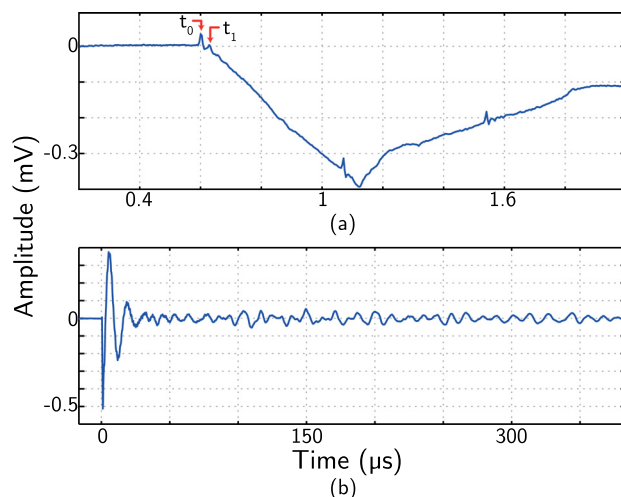
FIG. 7. (Color online) Typical signal measured by transmission in the Duralumin/epoxy/Duralumin structure: (a) at short arrival with a \sim 100 \mu\text{m} beam diameter to observe first reflections in the intermediate layer, (b) with a beam diameter of \sim 3 \text{mm} to enhance ZGV mode resonances.
