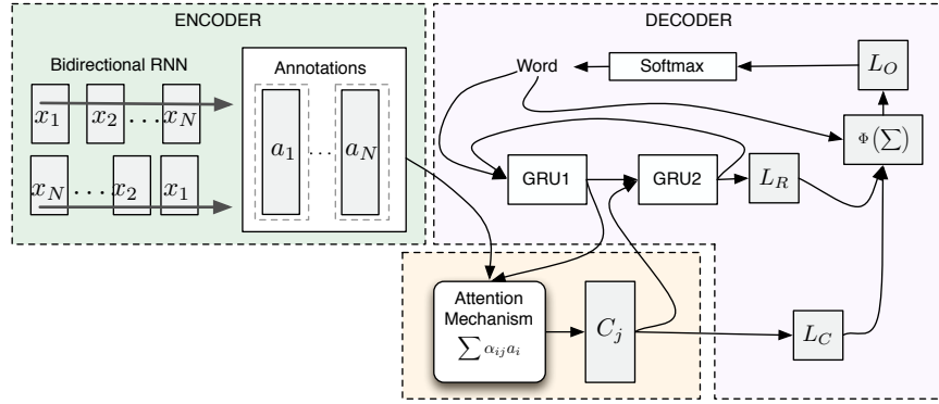
Fig. 1. Attention-based NMT system
